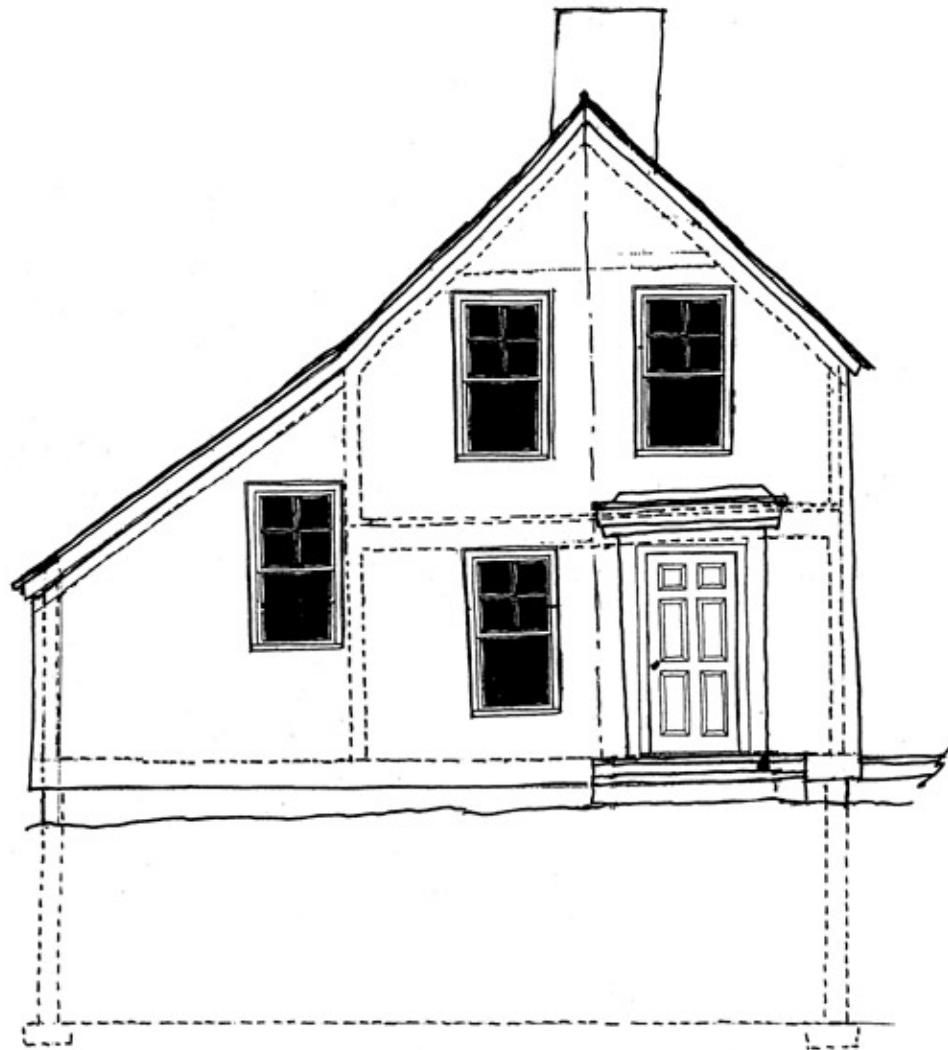
2 SOUTH ELEVATION 6 1/4" = 1'0"
