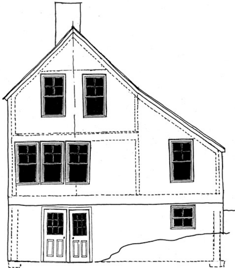
1 NORTH ELEVATION 6 1/4" = 1'0"
