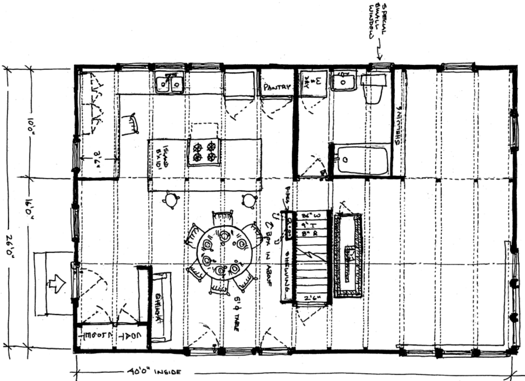
① MAIN FLOOR PLAN ② 1/4" = 10"
