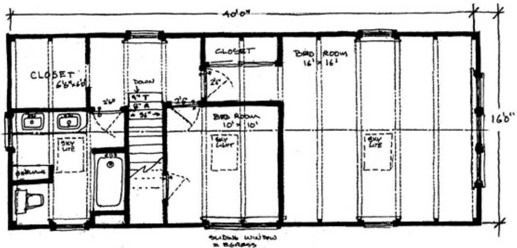
1 UPPER LEVEL PLAN \frac{3}{16}'' = 10''
