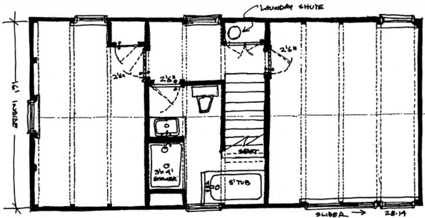
① 2ND FLOOR PLAN ② 1/4" = 1'0"
