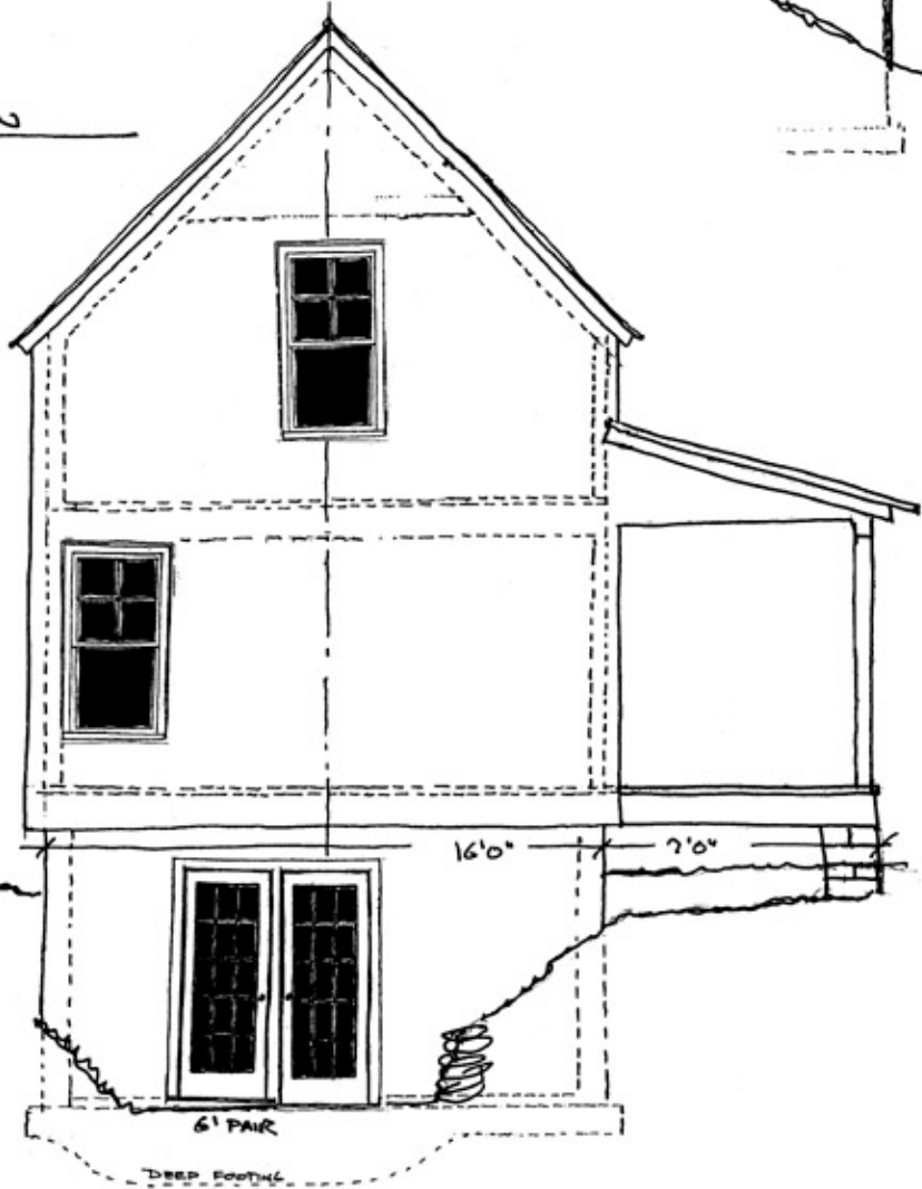
2 4 WEST ELEVATION \frac{1}{4}'' = 1'0''
