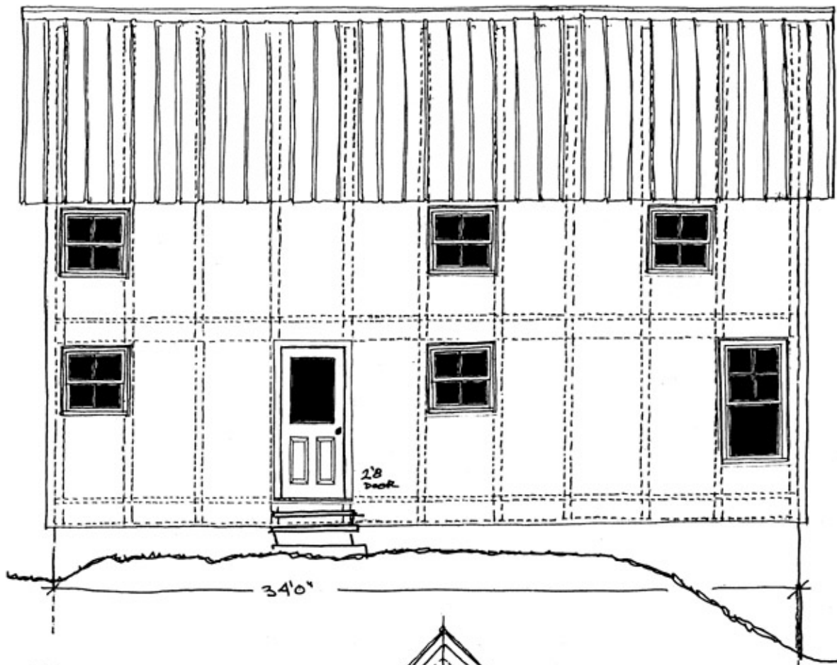
1 4 NORTH ELEVATION \frac{1}{4}'' = 1'0''
