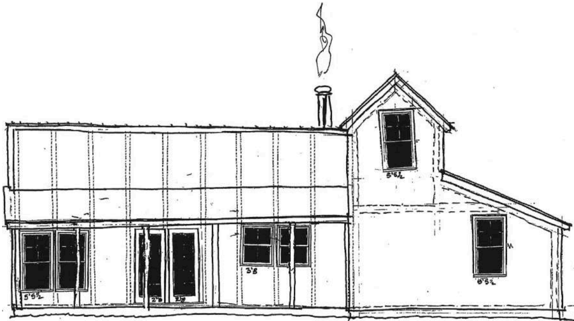
\frac{1}{1} EAST ELEVATION \frac{3}{16} = 1'0"
