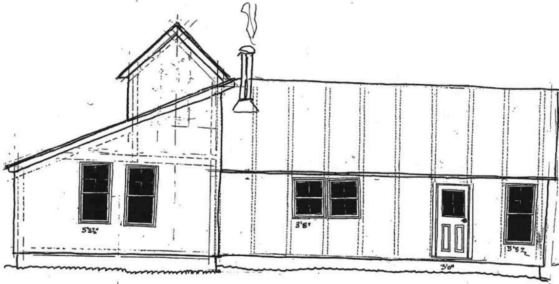
\frac{2}{3} WEST ELEVATION \frac{3}{16} = 10''
