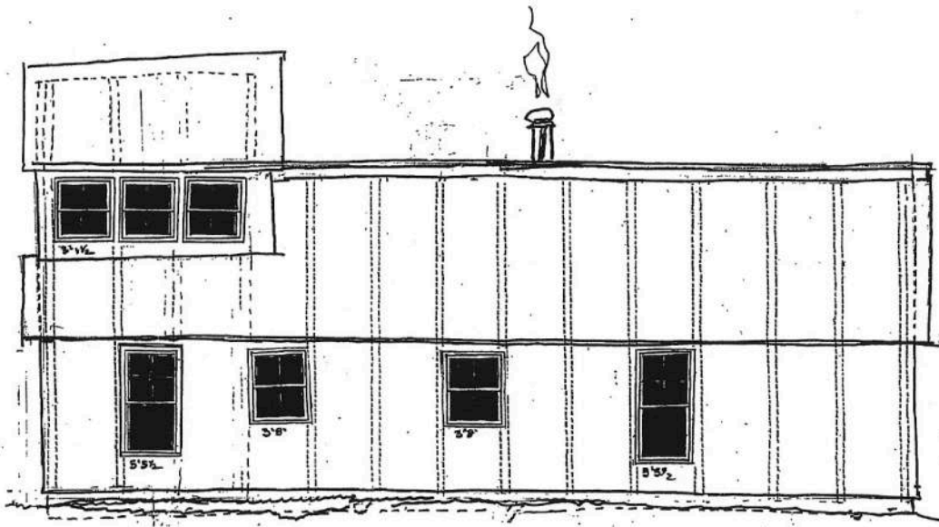
\frac{2}{1} NORTH ELEVATION \frac{3}{16} = 1'0"
