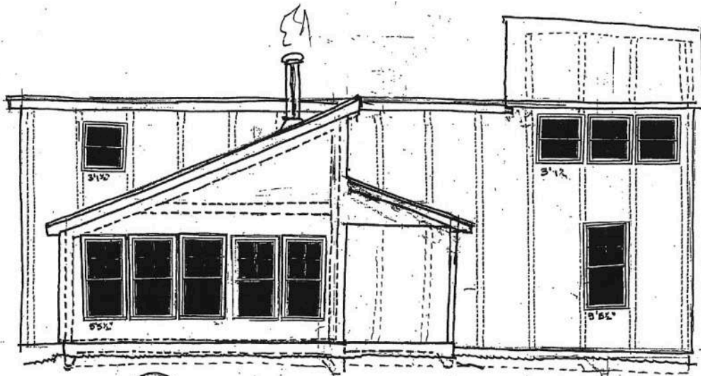
\frac{1}{3} SOUTH ELEVATION \frac{3}{16} = 10''
