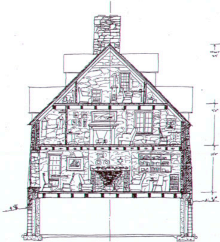
CROSS SECTION
